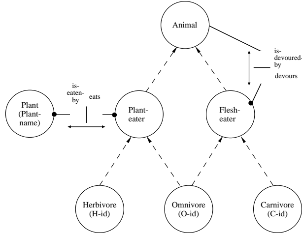
Figure 9: Another example of generalisation
