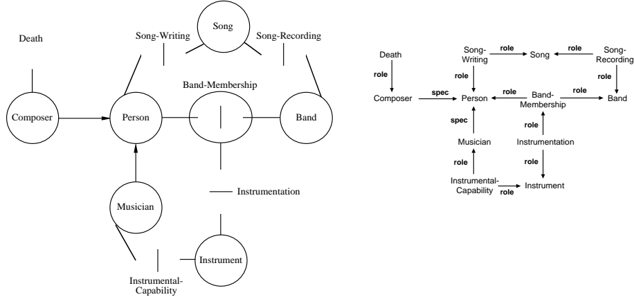
Figure 1: A NIAM data model and its representation as a type graph
