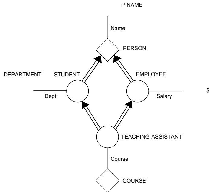
Figure 6: An example of a subtype hierarchy in IFO
