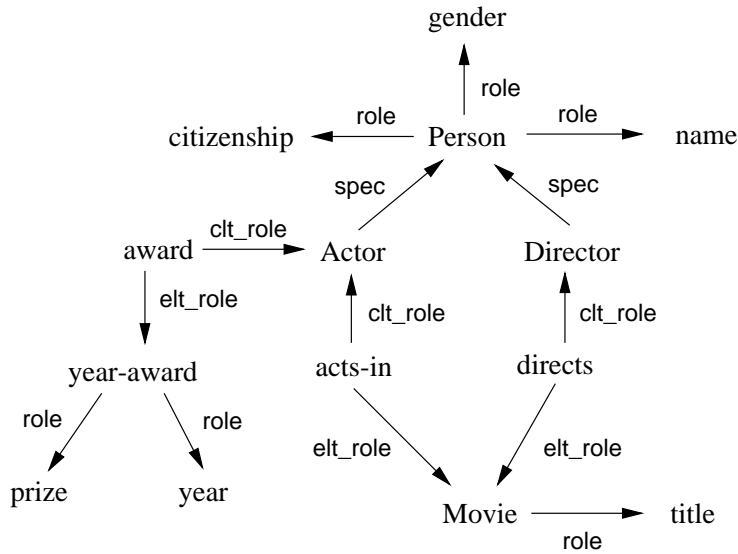
Figure 14: Type graph for OO type definitions
