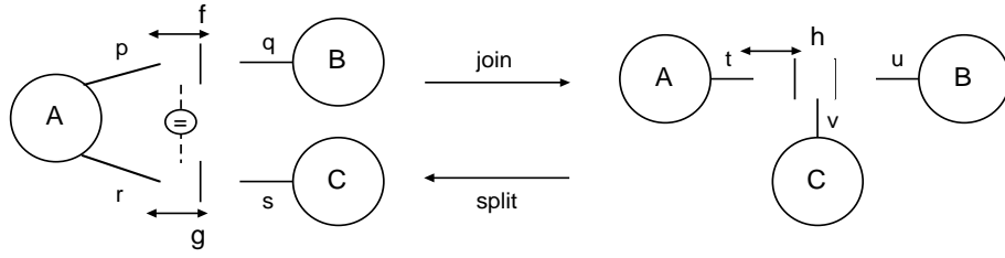
Figure 17: Illustration of the join/split transformation in NIAM
