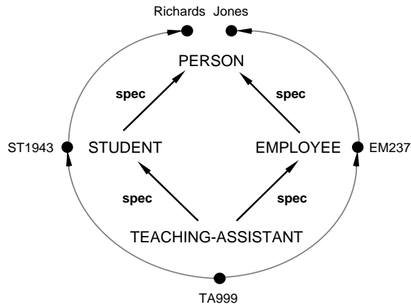
Figure 7: A non-commutative diagram
