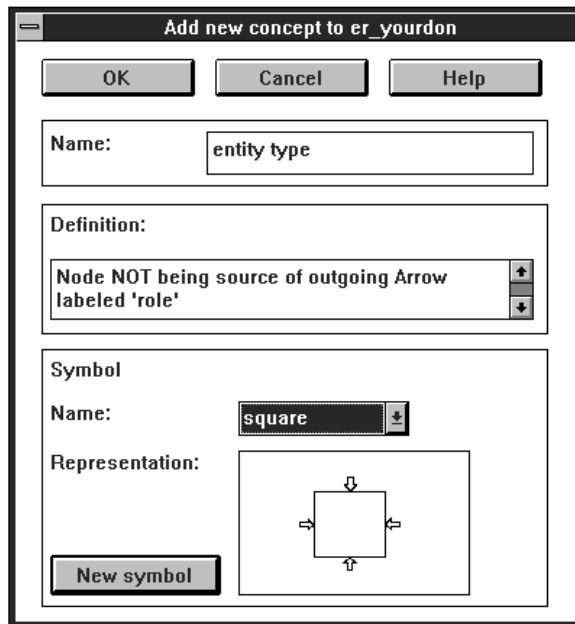
Figure 21: Defining the concrete representation of a concept
