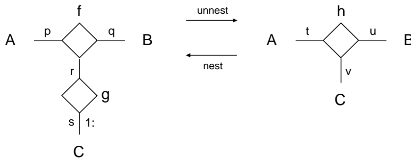
Figure 16: Illustration of the nest/unnest transformation in ER
