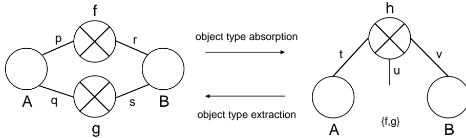
Figure 15: Illustration of the absorption/extraction transformation in IFO
