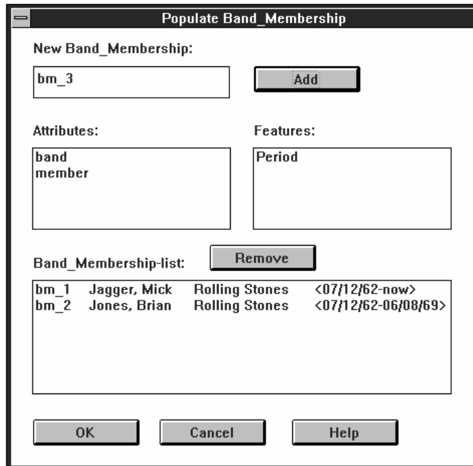
Figure 26: Populating an object type
