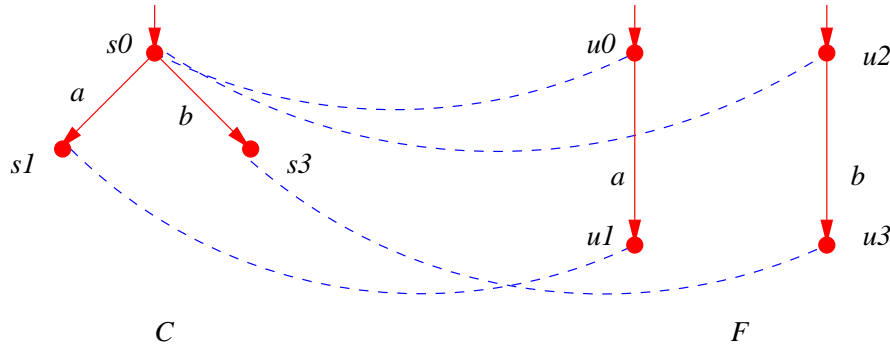
Figure 8: The need for backward simulations.
