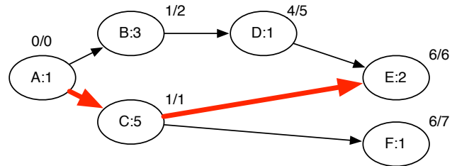
Fig. 1. Critical path analysis of a small task graph. Execution times are shown after the task names. The tasks are annotated with a/b where a is the earliest start and b is the latest start. The only critical path is A \rightarrow C \rightarrow E .
