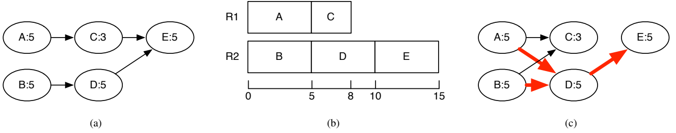
Fig. 3. Figure (a) shows a task graph, Figure (b) shows the non-delay interpretation of this task graph as a Gantt chart, and (c) shows the \mapsto relation as extracted from this Gantt chart by Algorithm 2.
