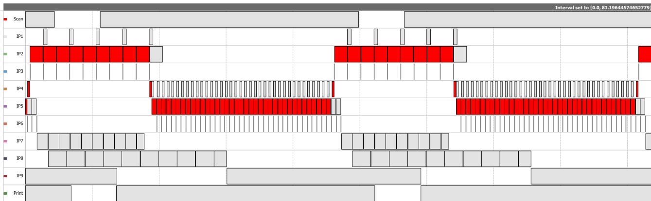
Fig. 6. A part of a trace of a COPY job which shows under-utilization of the scanner and printer hardware.
